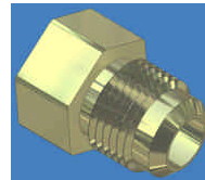
45° Flare 3/8"-24 to 7/8"-14
